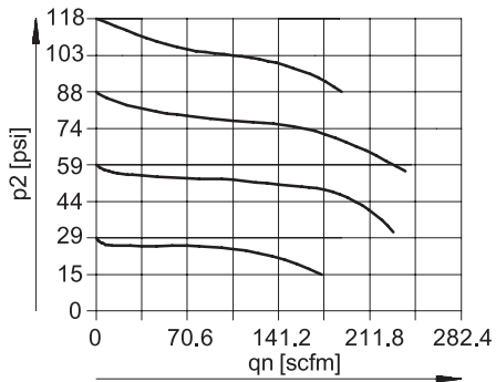
Standard flow rate q_n as a function of the outlet pressure p_2 (combination 6, grade of filtration 5 \mu\text{m} )
