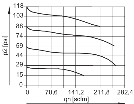
Standard flow rate q_n as a function of the output pressure p_2 (combination 6, grade of filtration 40 \mu\text{m} )
