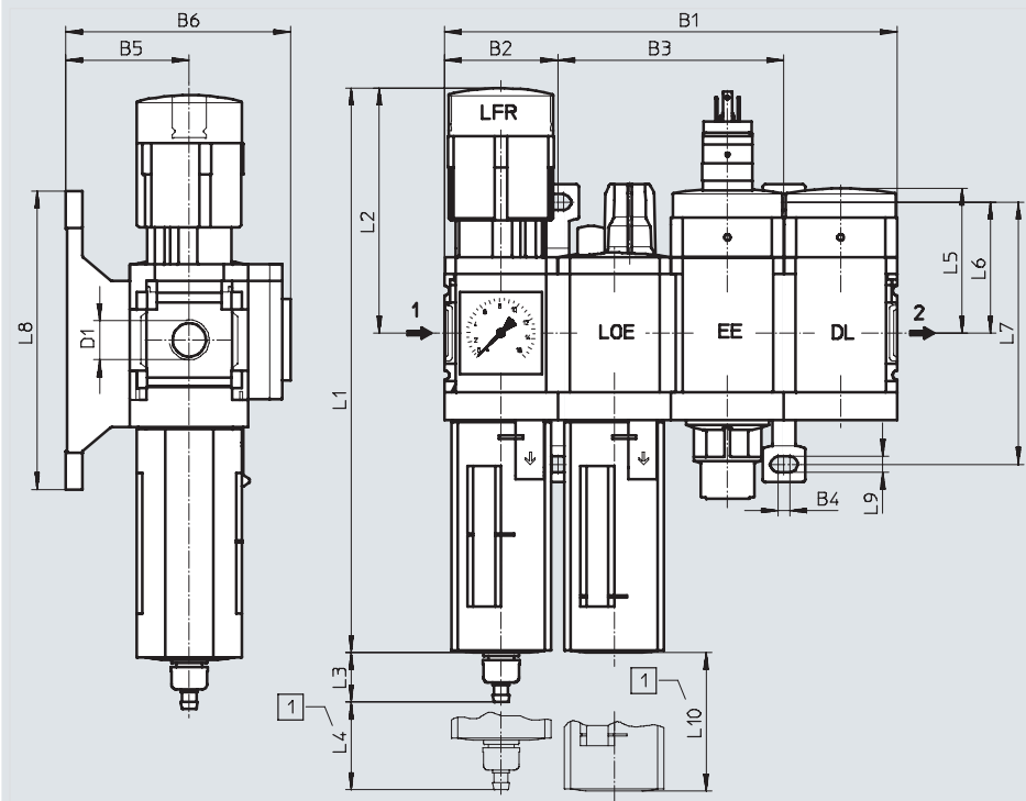
[1] Installation dimension
