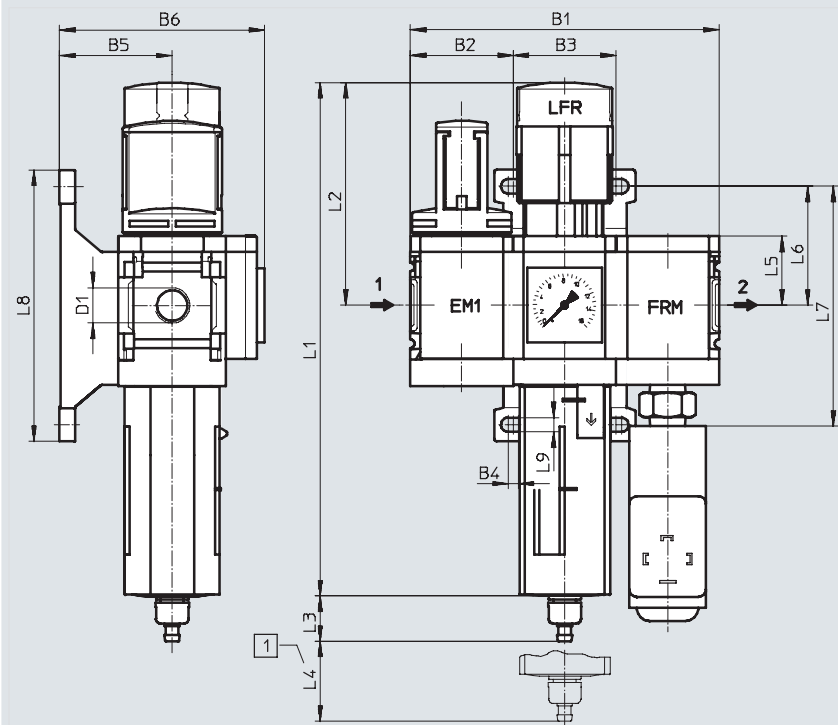
[1] Installation dimension
