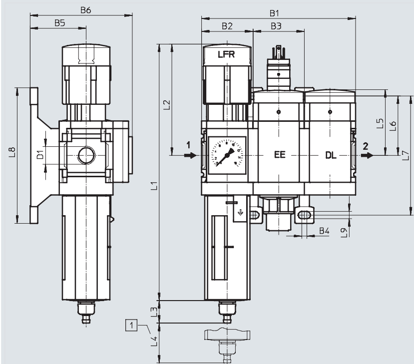
[1] Installation dimension
