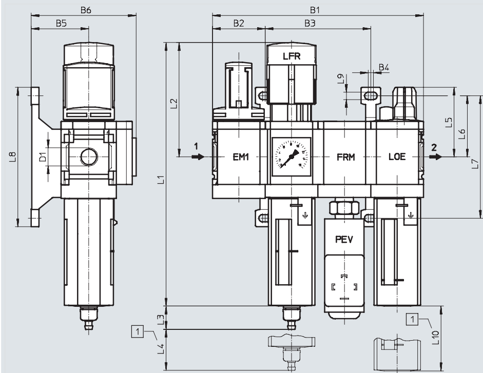
[1] Installation dimension
