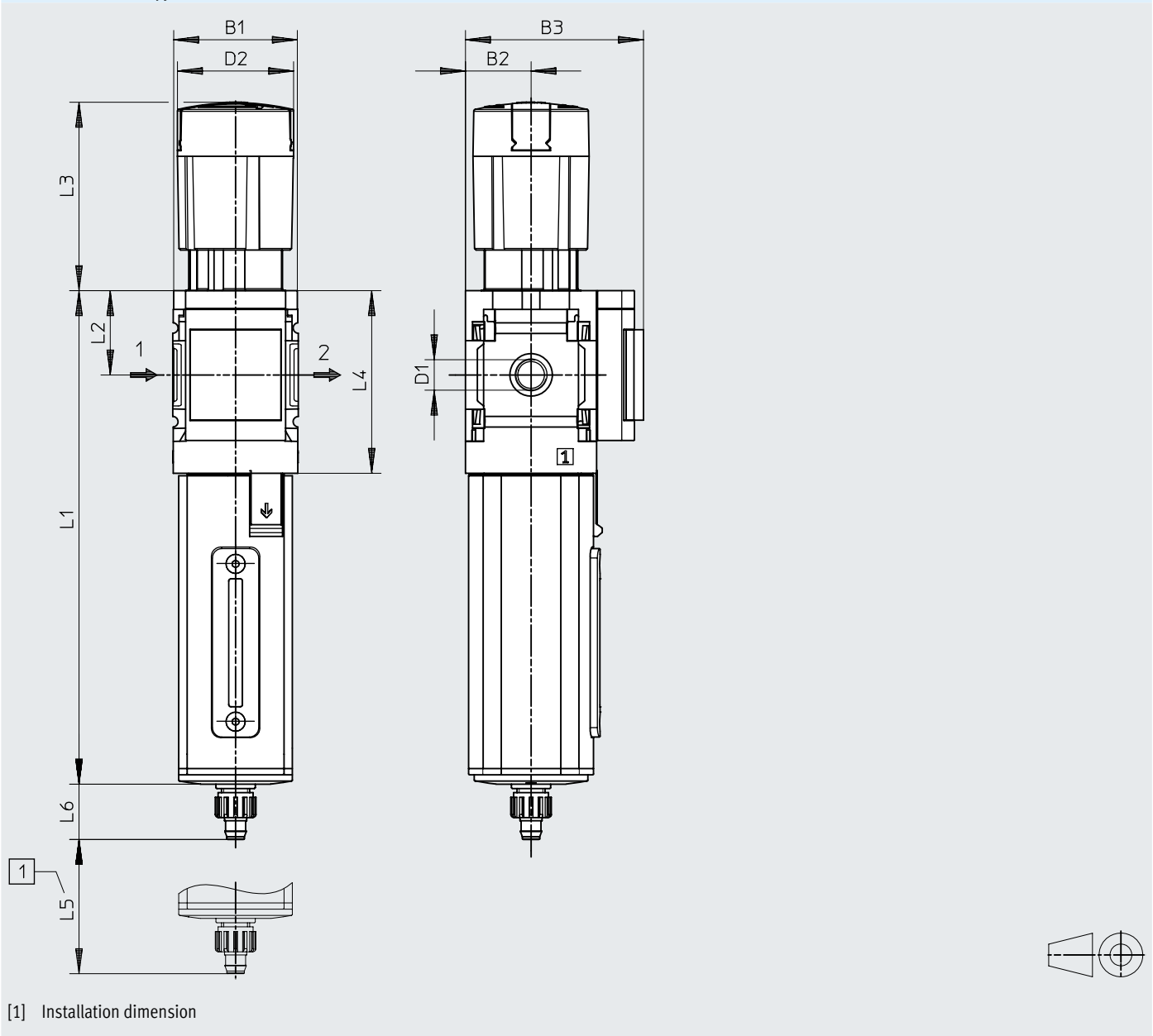
Dimensions – Basic type with metal bowl
