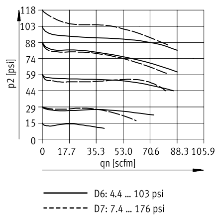
Normal flow rate q_n as a function of output pressure p_2 ( p_1 = 147 psi) - MS4N-LFR-1/4 (grade of filtration: 40 \mu\text{m} )
