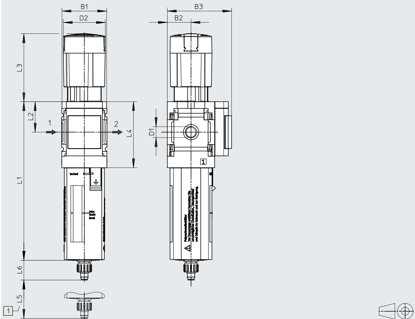
[1] Installation dimension
