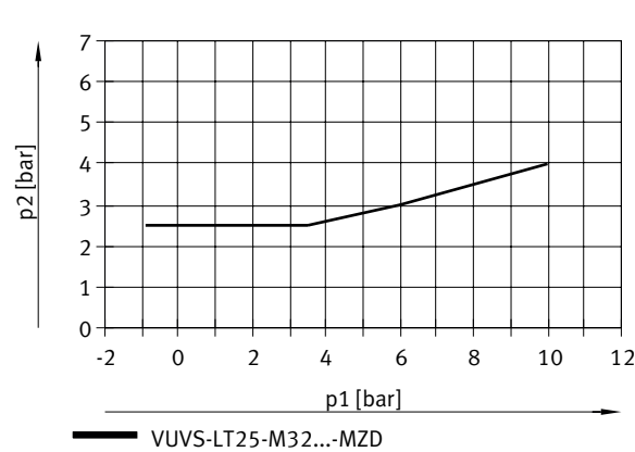
Size 25 – Pilot pressure p2 as a function of working pressure p1 with external pilot air supply
