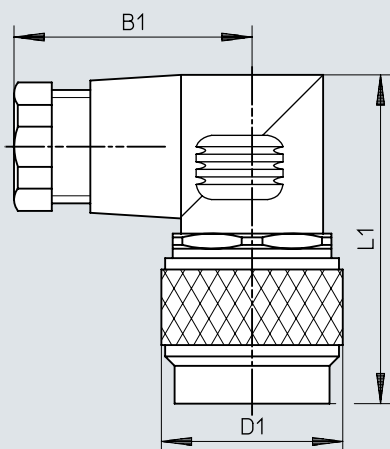
Dimensions – Angled plug socket
