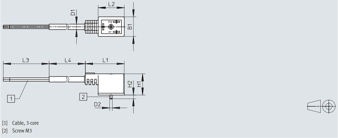
Dimensions – Connecting cable with PVC cable sheath
