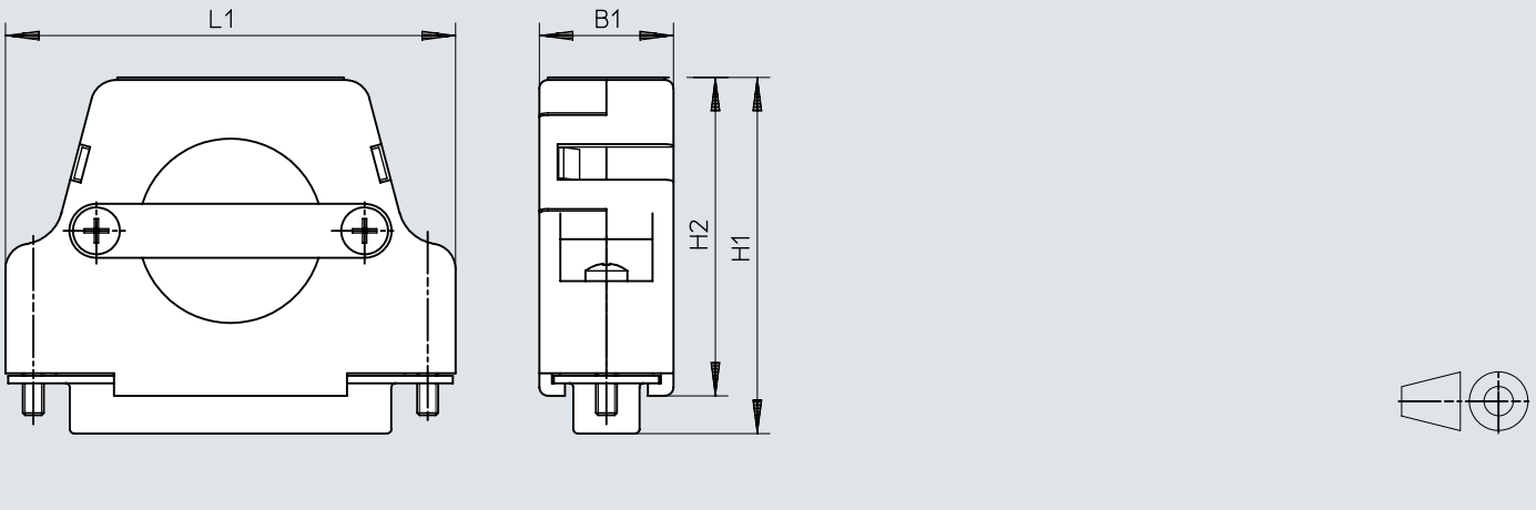
Dimensions – Plug socket
