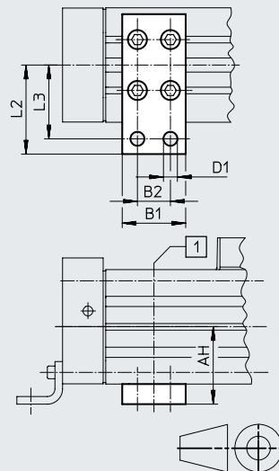
Piston Ø 32 ... 63
