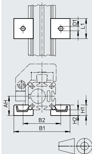
Piston Ø 18 and 25
