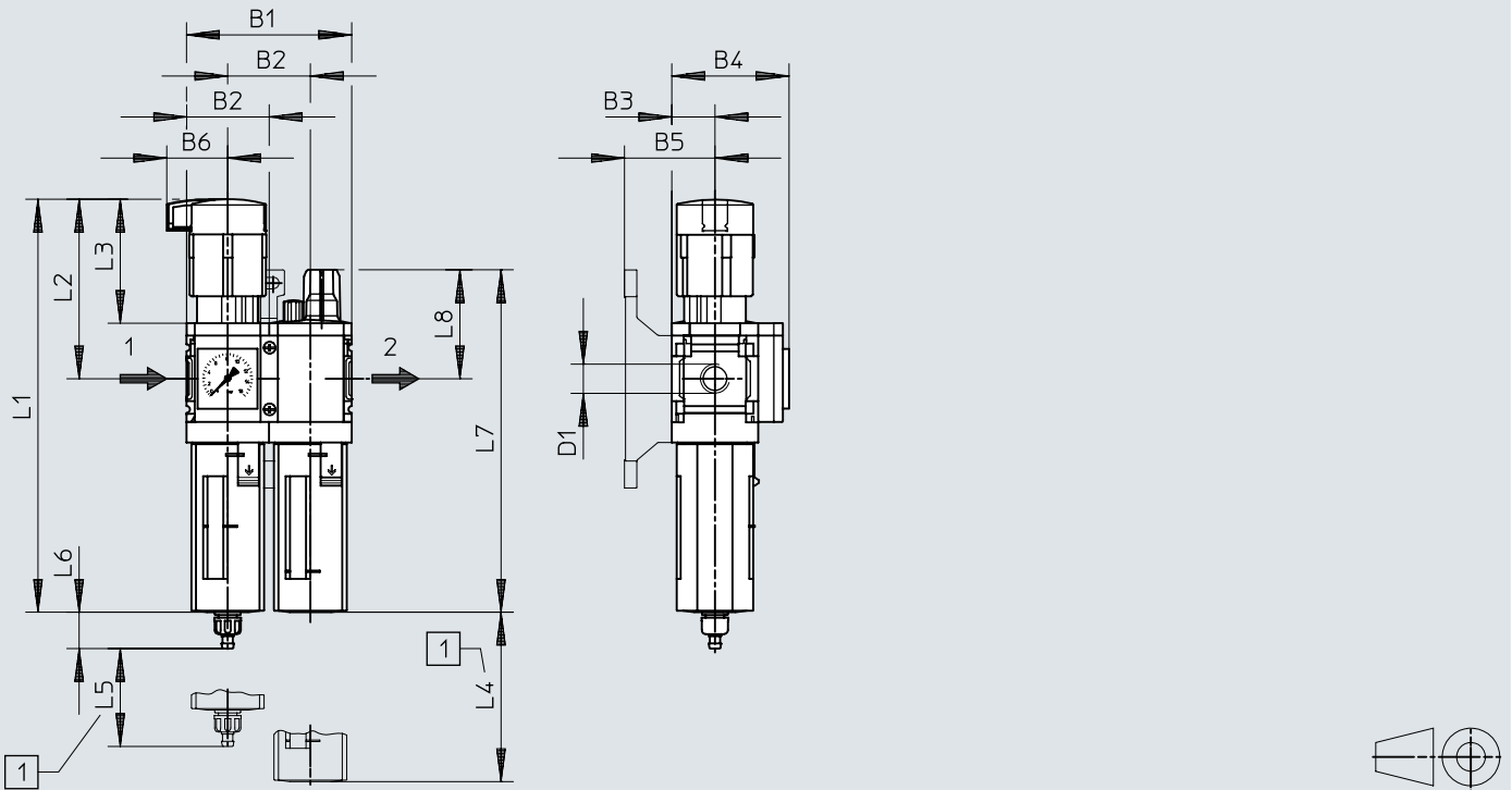
[1] Installation dimension
