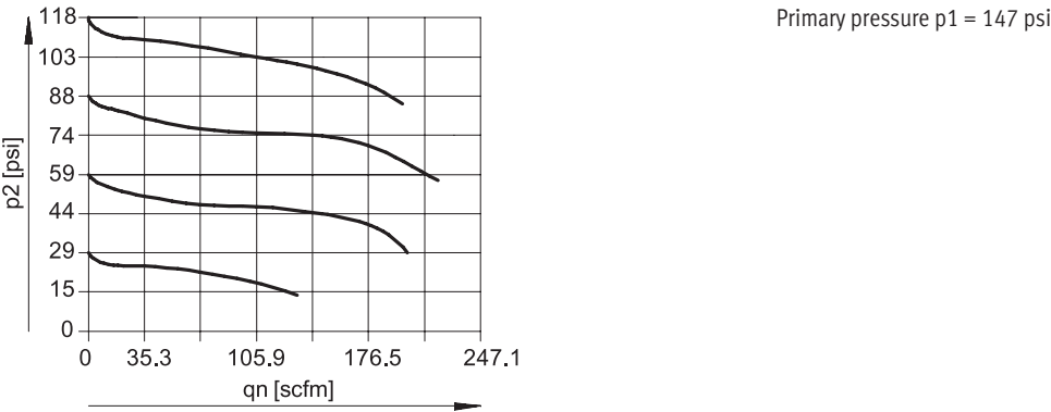
Normal flow qn as a function of output pressure p2 (MSB6N-1/2; pressure regulation range 7.4 ... 176 psi; grade of filtration 40 µm)
