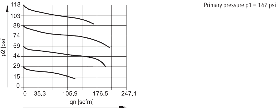
Normal flow qn as a function of output pressure p2 (MSB6N-1/2; pressure regulation range 7.4 ... 176 psi; grade of filtration 5 µm)
