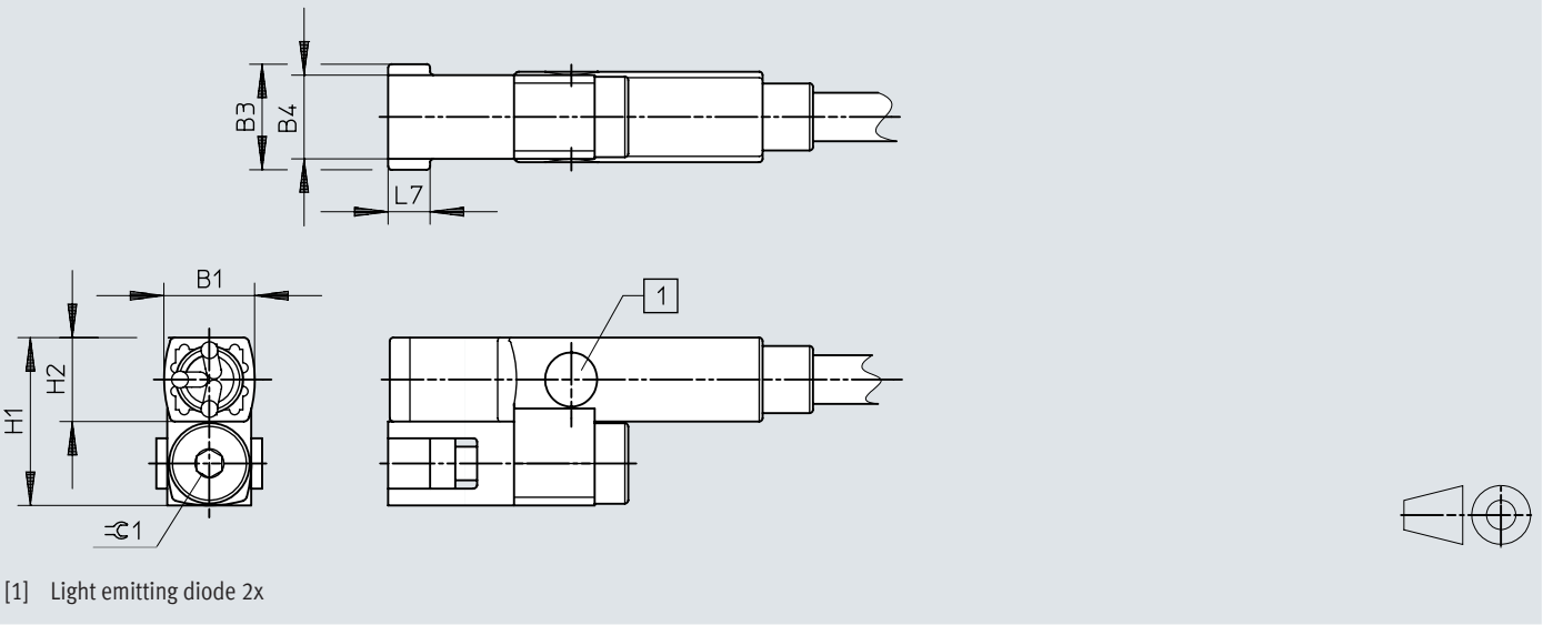
Dimensions – SMT-8-G
