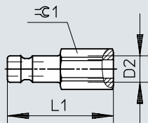
Dimensions – Quick coupling plug KS3, female thread
