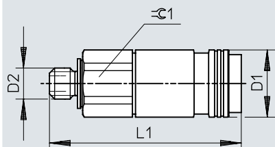
Dimensions – Coupling socket KD1, male thread
