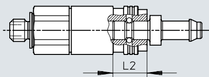
Dimensions – Plug-in coupling KD1/KS1, insertion depth
