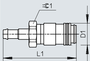
Dimensions – Coupling socket KD4, barbed fitting
