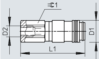
Dimensions – Coupling socket KD2, female thread
