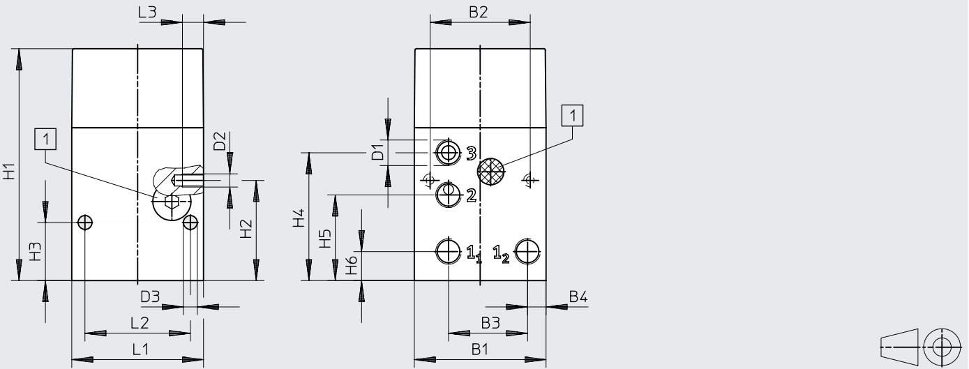
Dimensions – Control blocks for two-hand start
