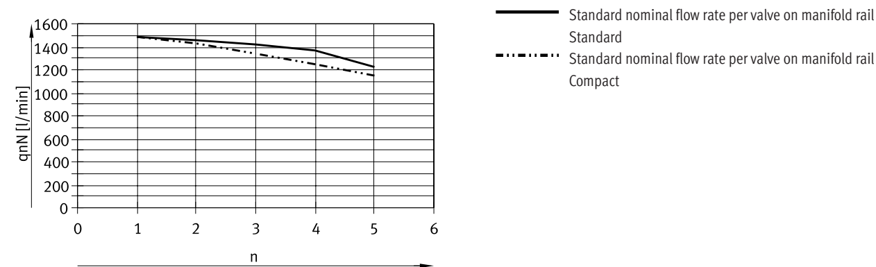
For 2x 3/2-way valves Both valve functions per valve position simultaneously in open switching position
