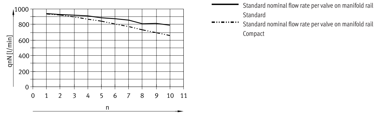
Size 25 – Standard nominal flow rate q_{nN} , with several valves n switched in parallel For 2x 3/2-way valves One valve function per valve position in open switching position
