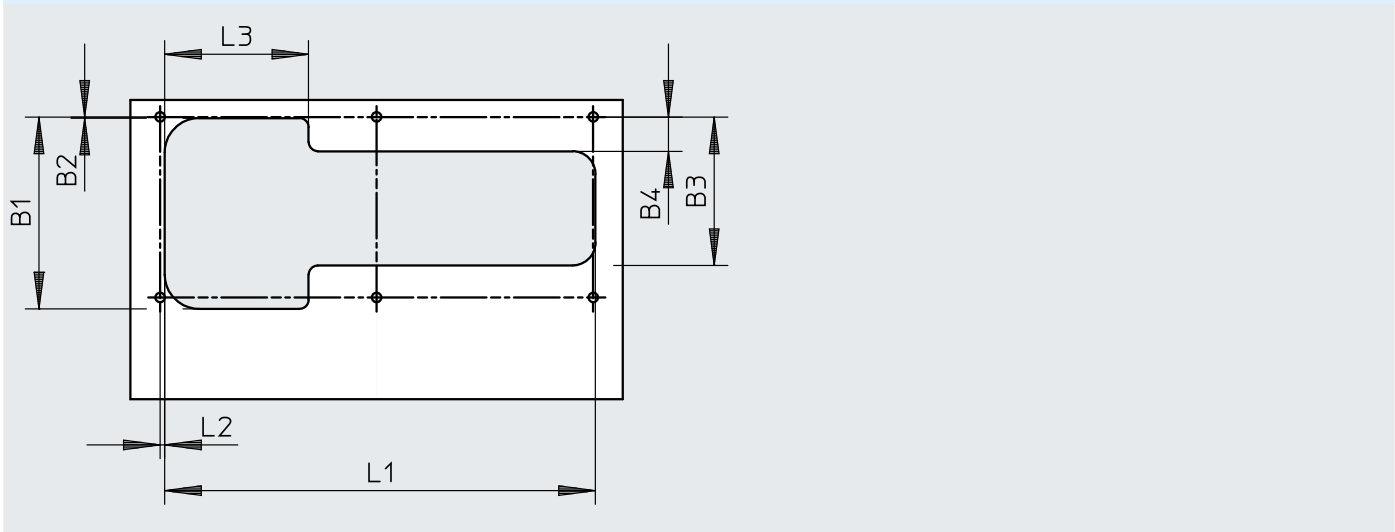
Dimensions – Recess for control cabinet installation, outlet direction underneath, size 18
