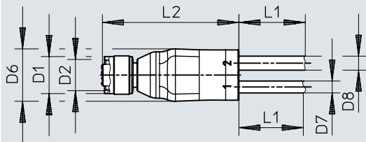
Dimensions – DUO cable NEDU-L1R2-V9-M12G8-E
