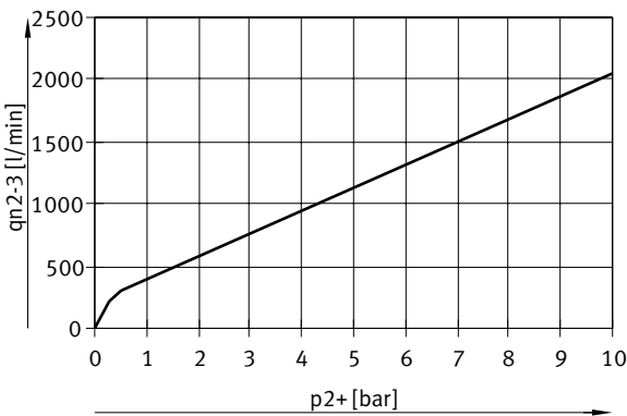
Flow rate q_n from 2 → 3 as a function of output pressure p_2 , VPPX-8F-...-0L10H-... (10 bar)
