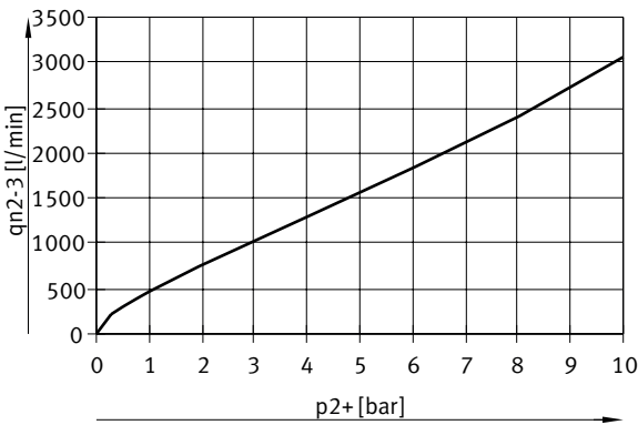
Flow rate q_n from 2 → 3 as a function of output pressure p_2 , VPPX-8L/F-...-0L10H-... (10 bar)
