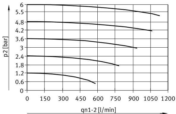
Flow rate q_{n1-2} from 1 -> 2 as a function of excess output pressure p_2 , VPPM-6L/F-...-0L6H-... (6 bar)
