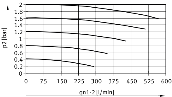
Flow rate qn from 1 -> 2 as a function of excess output pressure p2, VPPM-6L/F-...-0L2H-... (2 bar)
