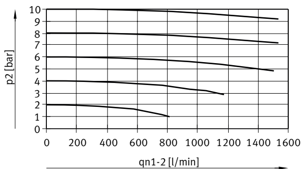
Flow rate q_{n1-2} from 1 -> 2 as a function of excess output pressure p_2 , VPPM-6L/F-...-0L10H-... (10 bar)
