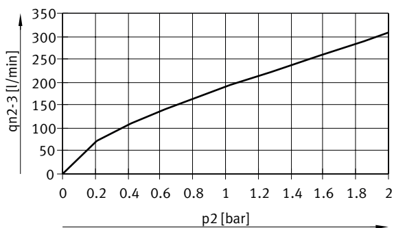
Flow rate q_{n2-3} from 2 -> 3 as a function of excess output pressure p_2 , VPPM-6L/F-...-0L2H-... (2 bar)
