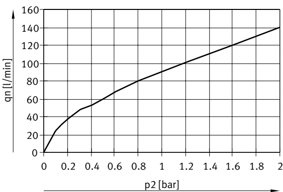
Flow rate qn as a function of output pressure p2, VPPE-3-1-1/8-2-..., qn 2 -> 3
