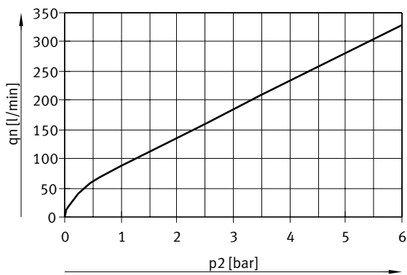
Flow rate q_n as a function of output pressure p_2 , VPPE-3-1-1/8-6-..., q_n 2 -> 3
