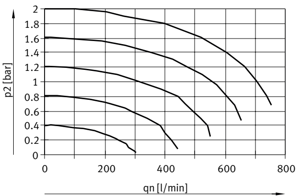
Flow rate qn as a function of output pressure p2, VPPE-3-1-1/8-2-..., qn 1 -> 2
