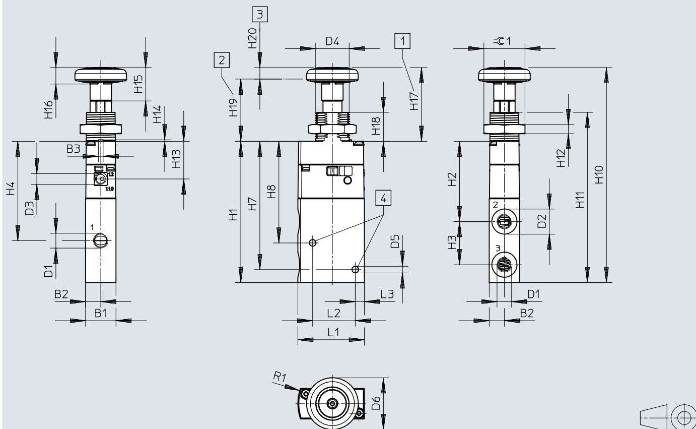
Dimensions – 3/2-way valve, pushbutton valve
