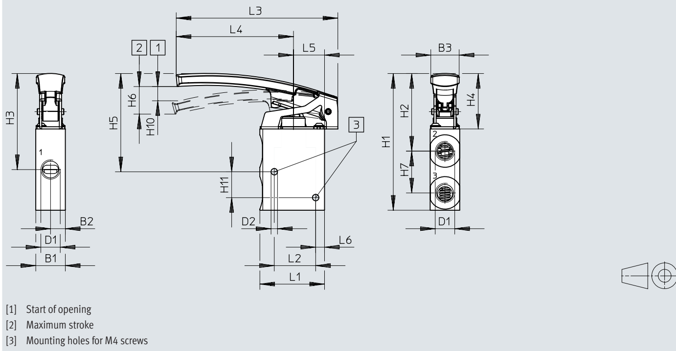
Dimensions – 3/2-way valve, finger lever valve
