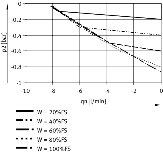
VEAB-....D14-..., output pressure 2 (pressure regulation range) -1 ... -0.005 bar, flow rate qn from 3 → 2 depending on output pressure p2
