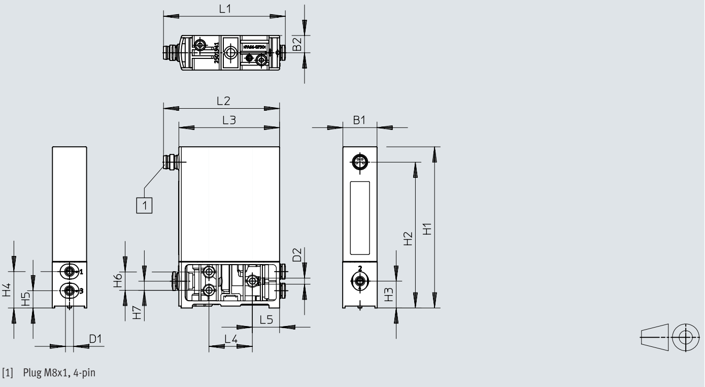
Dimensions – In-line valve
