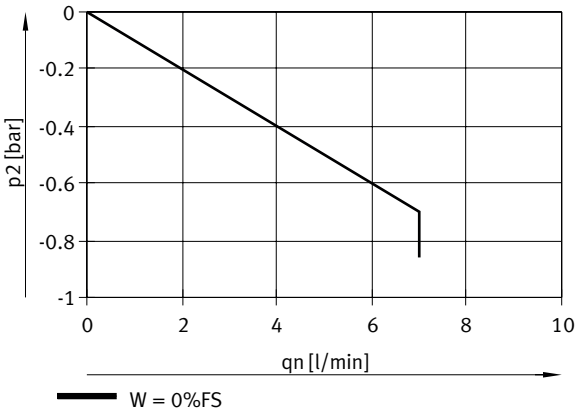
VEAB-....D14-..., output pressure 2 (pressure regulation range) -1 ... -0.005 bar, flow rate qn from 1 → 2 depending on output pressure p2
