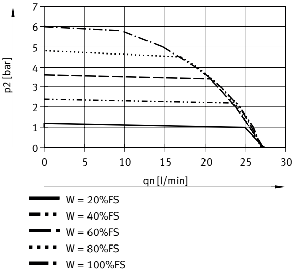
VEAB-....D9-..., output pressure 2 (pressure regulation range) 0.03 ... 6 bar, flow rate qn from 1 → 2 depending on output pressure p2
