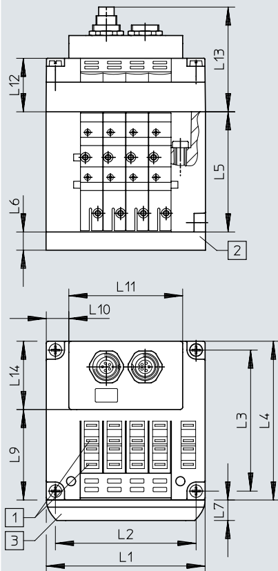
Valve terminal with installation system CPI – CPV10/14
