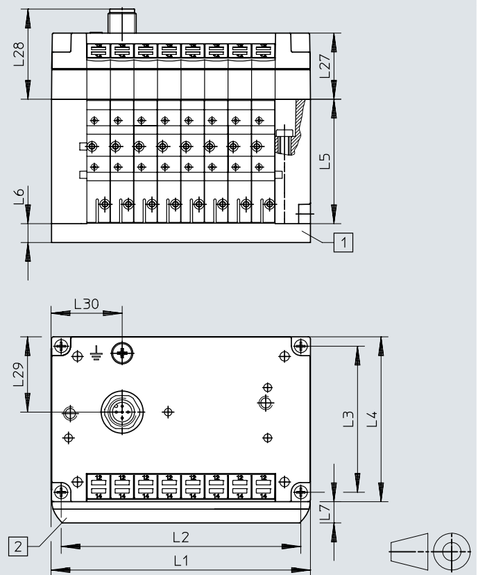
Valve terminal with I-Port interface/IO-Link® – CPV10/14
