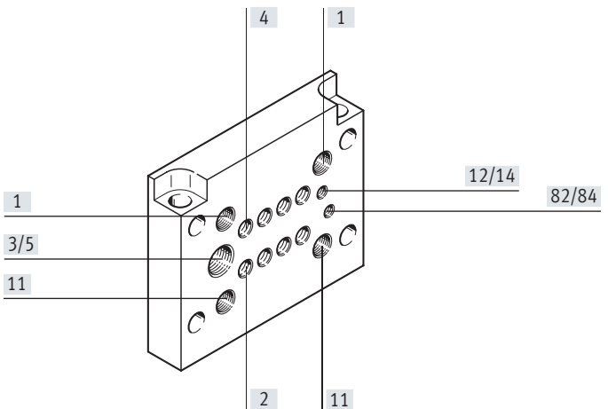
Pneumatic multiple connector plate
