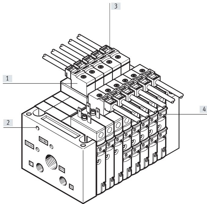
Valve manifold assembly CPV with individual connection
