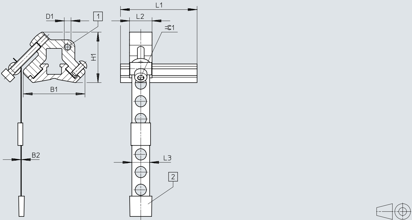
Dimensions – Mounting kit SMBR-8-8/100-S6
