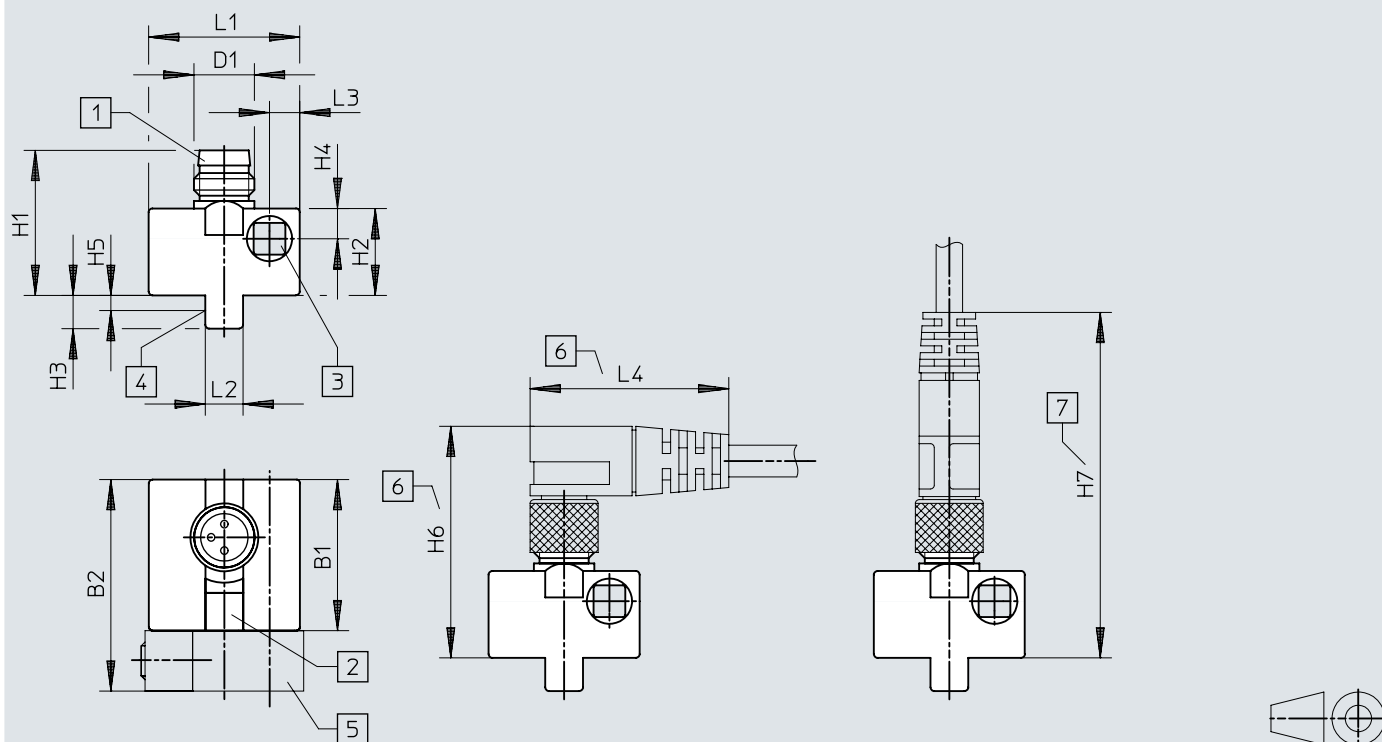
Dimensions – SMT0-8E-...-S-LED-24 – Plug M8x1
