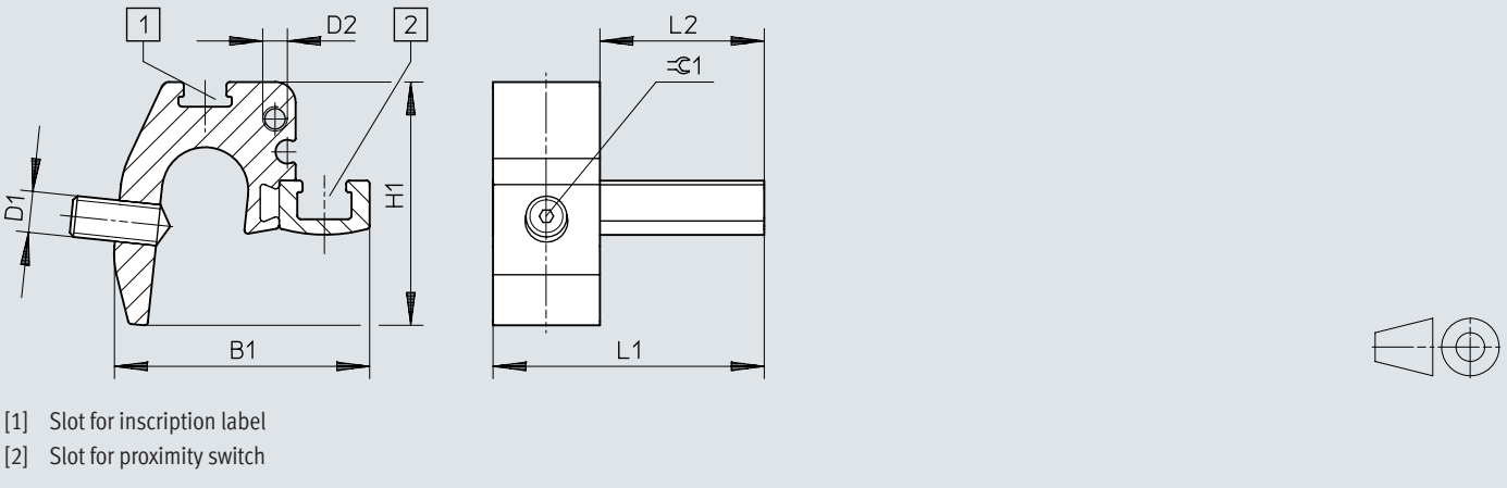
Dimensions – Mounting SMBZ-8-32/100
