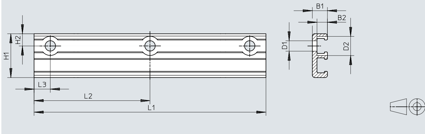
Dimensions – Sensor bracket SIEZ-8M
