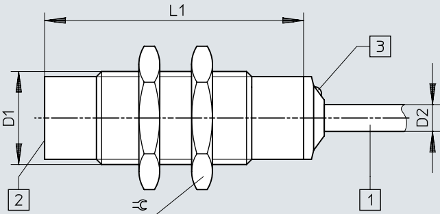
Dimensions – M18, partially flush mounted, cable
