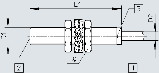
Dimensions – M8, flush mounted, cable
