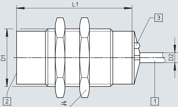
Dimensions – M30, partially flush mounted, cable
