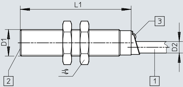
Dimensions – M12, flush mounted, cable
