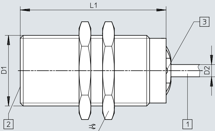
Dimensions – M30, flush mounted, cable
