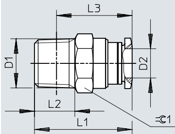
Dimensions – Push-in fitting QS, R thread
