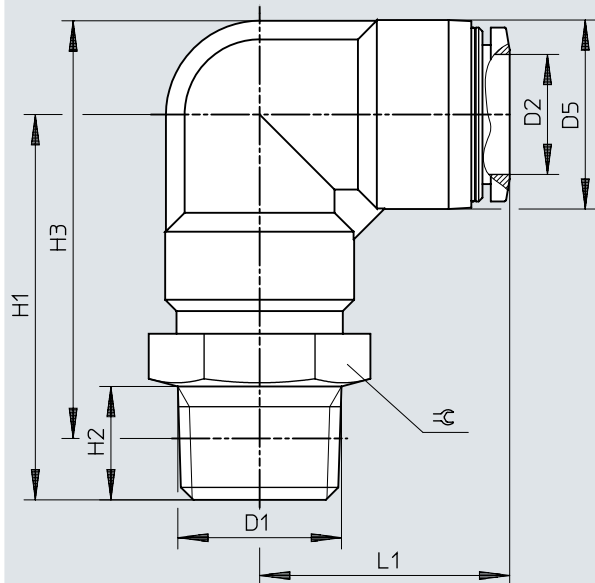
Dimensions – Push-in L-fitting QSL-...-16, R thread
