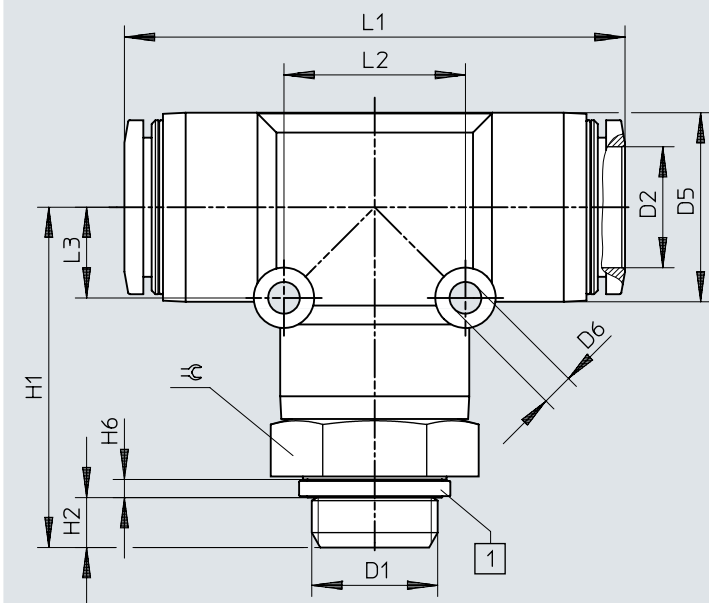
Dimensions – Push-in T-fitting QST-...-16, G thread with sealing ring
