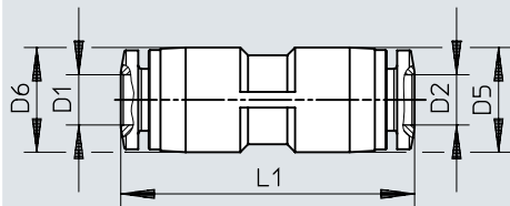
Dimensions – Push-in connector QS
