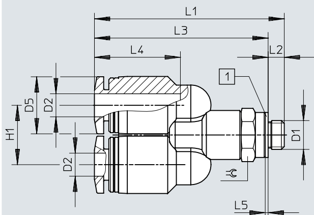
Dimensions – Push-in Y-fitting QSY, metric thread with sealing ring
