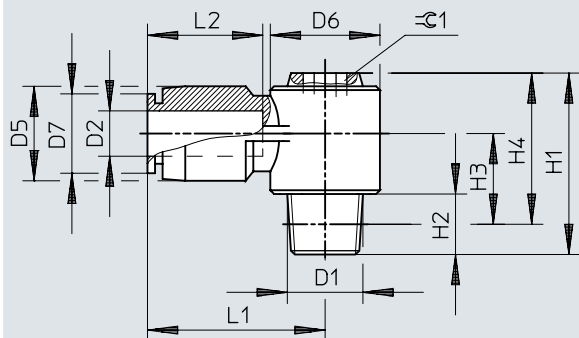
Dimensions – Push-in L-fitting QSLV-...-I, R thread
