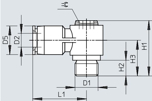
Dimensions – Push-in L-fitting QSLV-...-I, G thread
