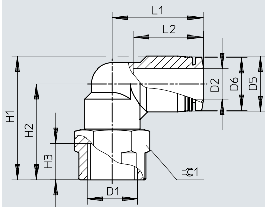
Dimensions – Push-in L-fitting QSLF, G thread
