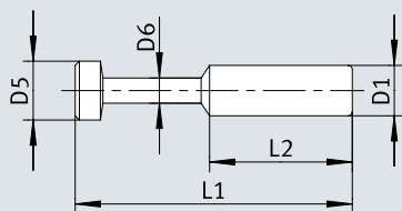
Dimensions – Blanking plug QSC-...6H/8H/10H/12H/16H
