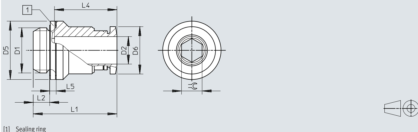
Dimensions – Push-in fitting QS-...-I, G-thread
