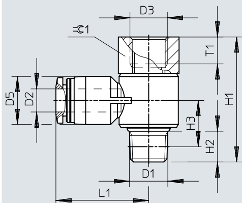
Dimensions – Push-in T-fitting QSTF, R thread
