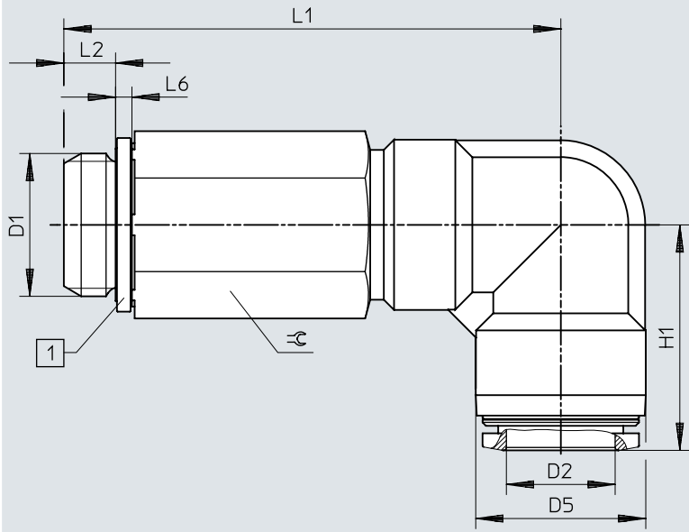
[1] Sealing ring
