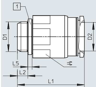
Dimensions – Push-in fitting QS-G3/8-16, G thread with sealing ring
