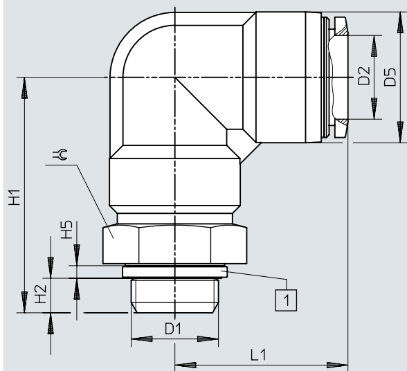
Dimensions – Push-in L-fitting QSL-...-16, G thread with sealing ring
