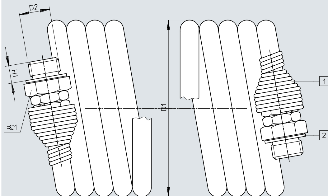
Dimensions – Spiral plastic tubing PPS
