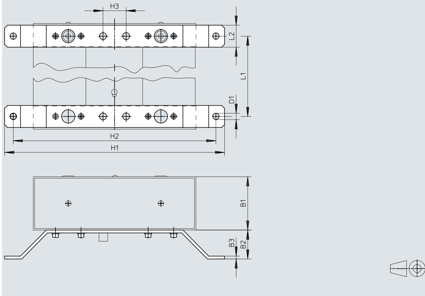
Dimensions – Wall mounting kit ABMW
