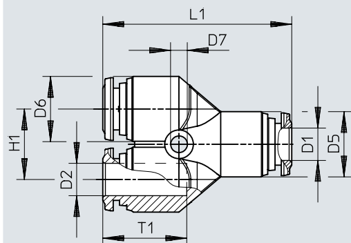
Dimensions – Push-in Y-connector NPQR-Y
