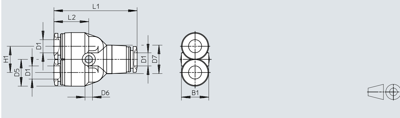
Dimensions – Push-in Y-connector NPQP-Y
