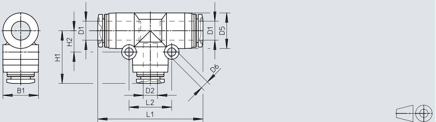
Dimensions – Push-in T-connector NPQP-T, reducing
