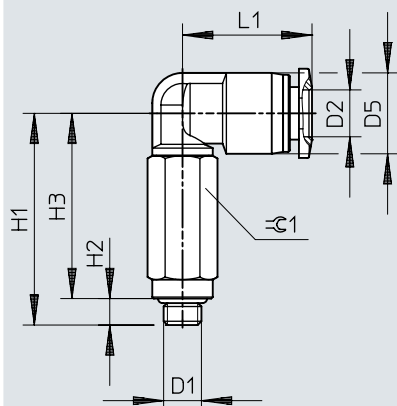
Dimensions – Push-in L-fitting, long, NPQE-LL, M thread
