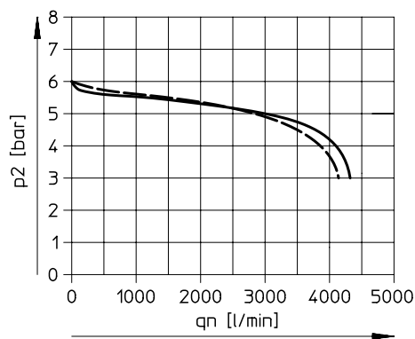
MS6-LR-1/2
