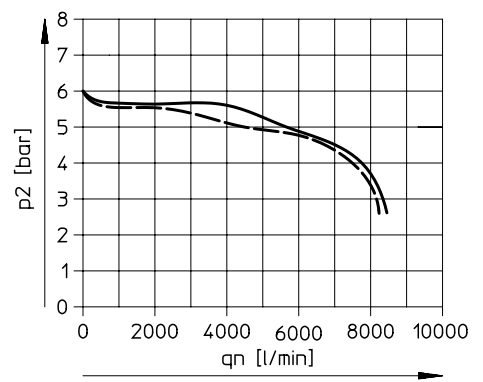
MS6-LR-3/8
