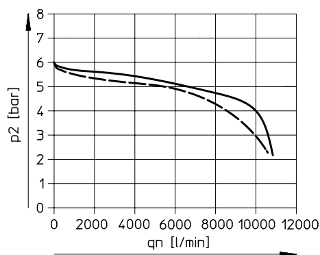
MS6-LR-1/2
