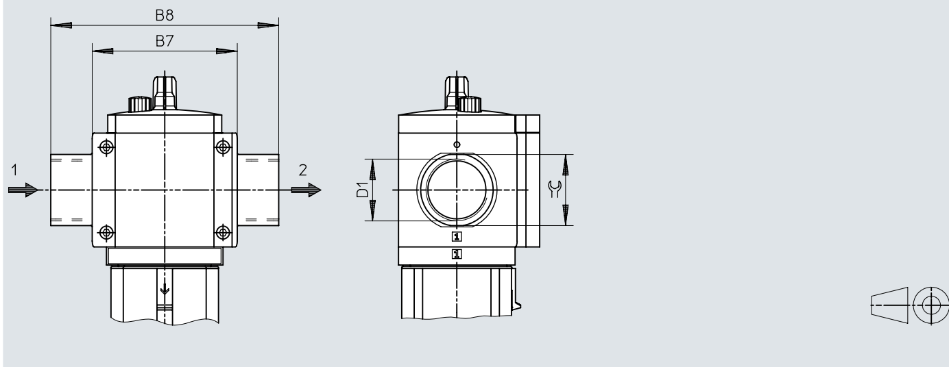
Dimensions – MS9, connecting plate
