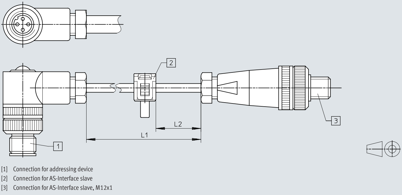
Dimensions – Addressing cable KASI-ADR
