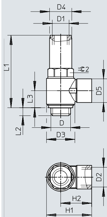
Dimensions – Threaded connection HGL-1/2-B
