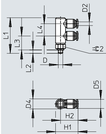
Dimensions – Push-in connector HGL-M5
