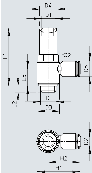
Dimensions – Push-in connector HGL-1/2
