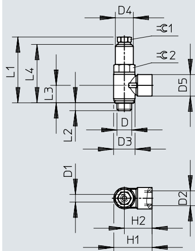
Dimensions – Threaded connection HGL-1/8-B, HGL-1/4-B, HGL-3/8-B
