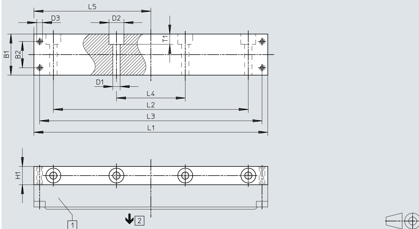
Dimensions – Foot mounting HBEV
