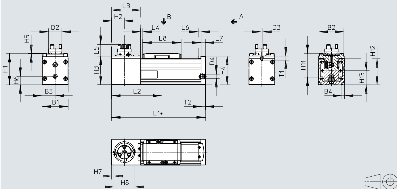
Dimensions – Toothed belt axes ELGC-TB-KF
