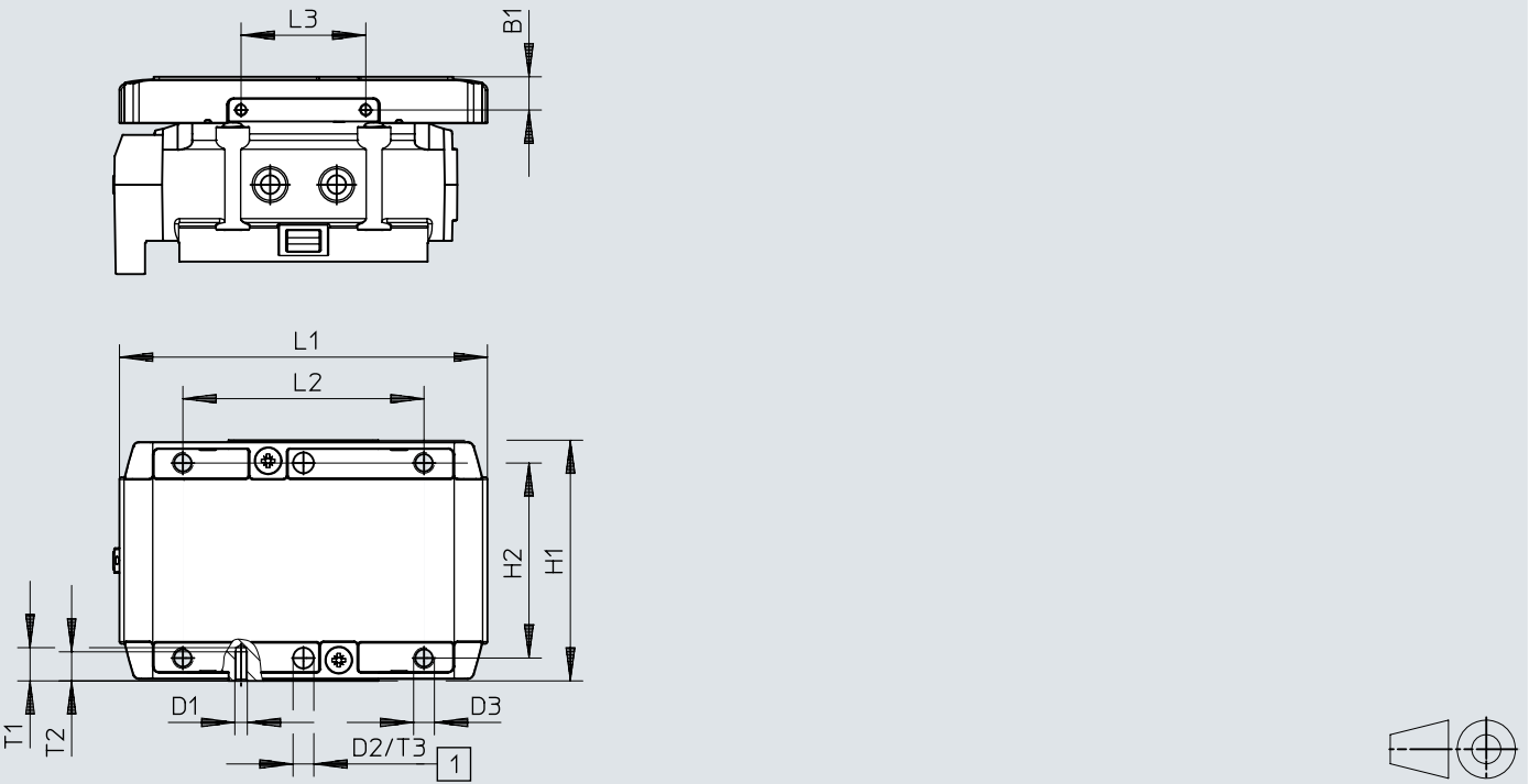
Dimensions – Toothed belt axes ELGC-TB-KF, size 60 (slide)
