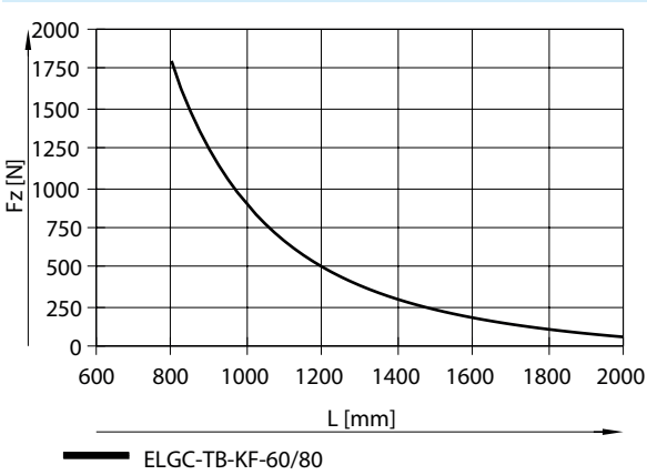
Max. permissible support spacing L (without profile mounting) as a function of force Fz for sizes 60/80
