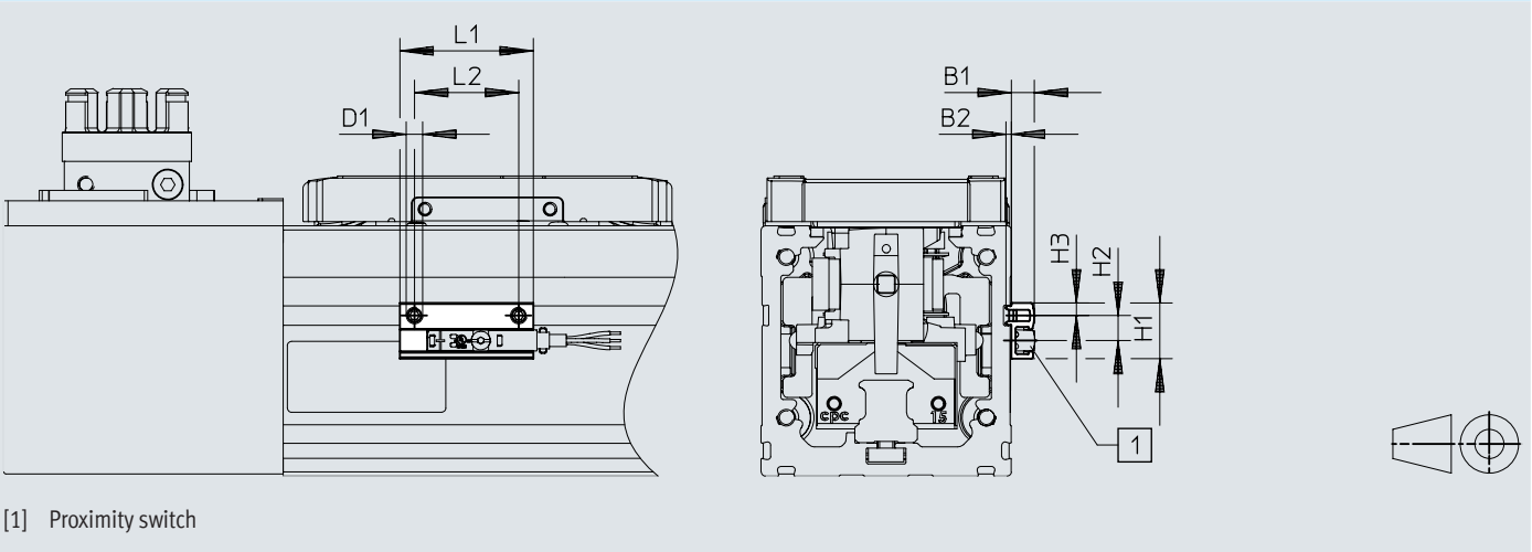
Dimensions – Sensor bracket EAPM-L2-SH
