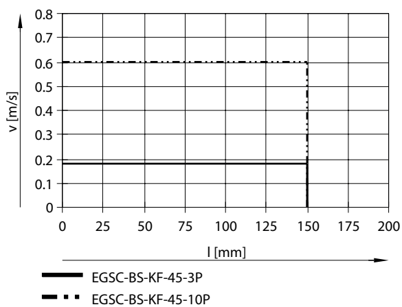
Speed v as a function of stroke l for size 45
