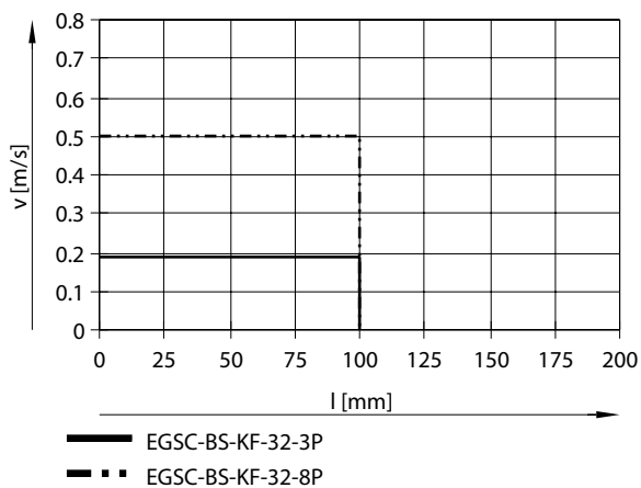
Speed v as a function of stroke l for size 32
