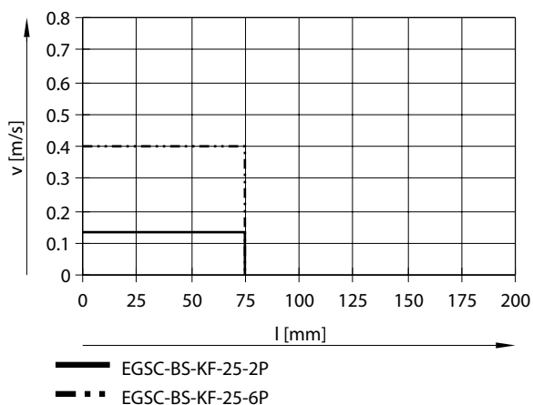
Speed v as a function of stroke l for size 25
