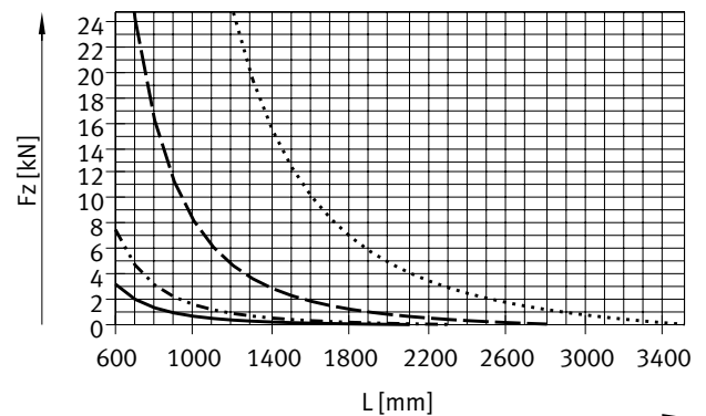
Force F_z
