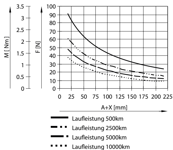
Payload F and torque M as a function of projection A for EAGF-P2-KF-32 with EPCC
