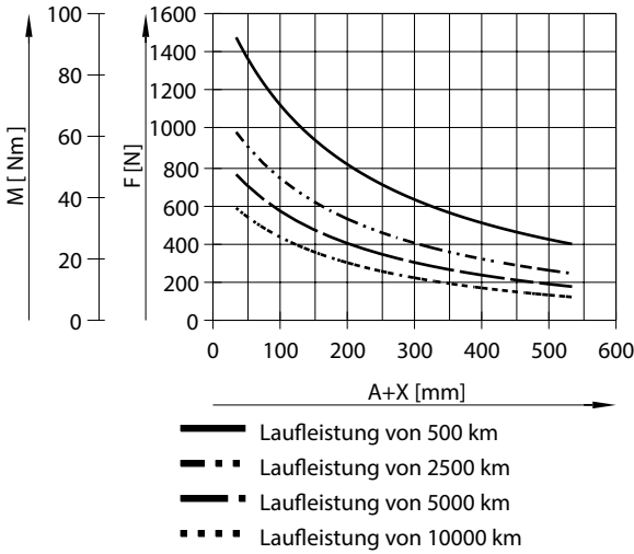
Payload F and torque M as a function of projection A for EAGF-V2-KF-80 with ESBF
