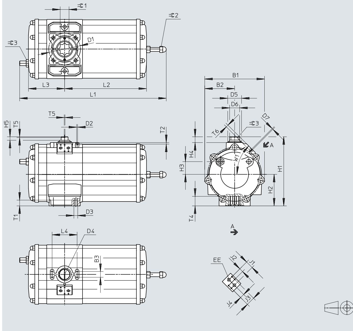
Dimensions – Size 1440, single-acting
