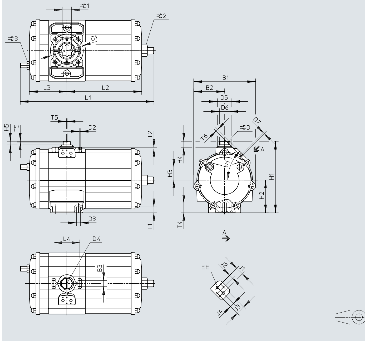
Dimensions – Size 2880, double-acting
