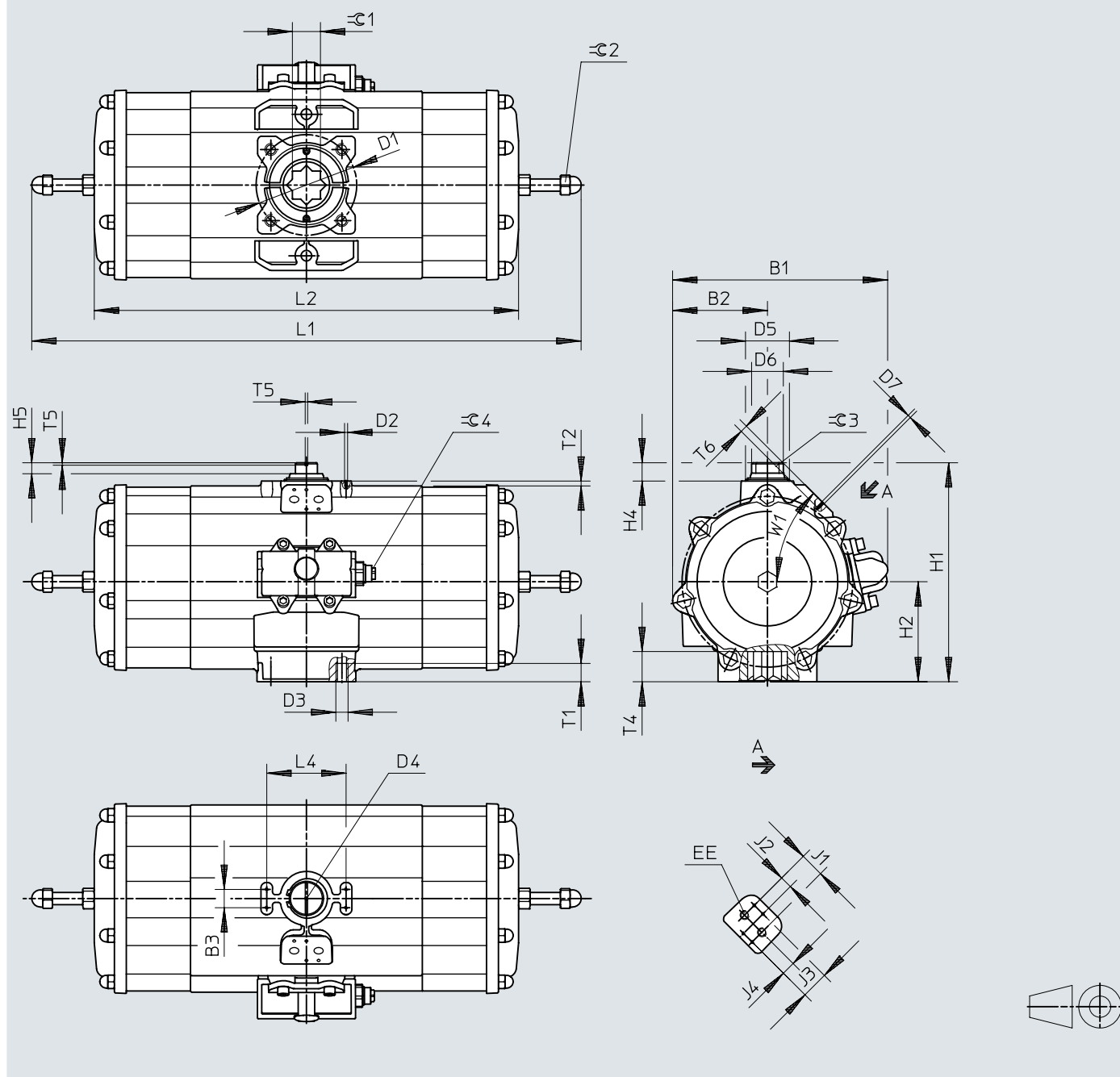
Dimensions – Size 2880, single-acting
