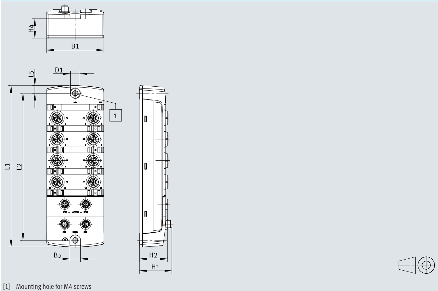
[1] Mounting hole for M4 screws
