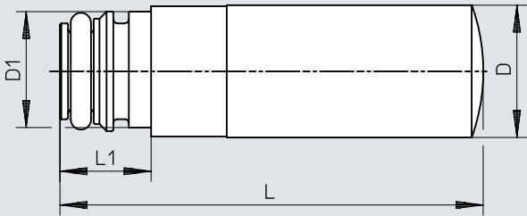
Dimensions – Cartridge 10 mm
