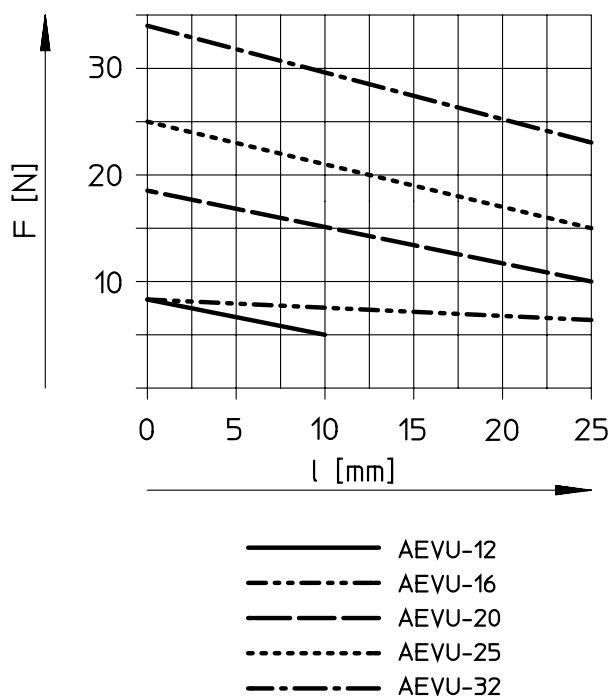
Spring return force F as a function of stroke – AEVU-12 ... 32
